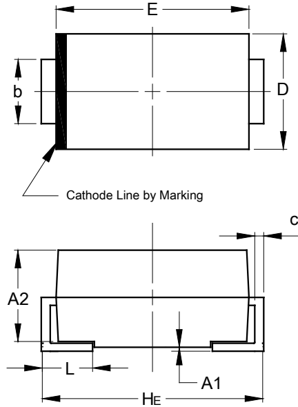
DO-214AC
